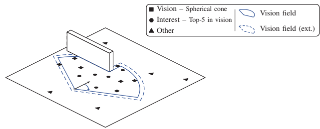
Figure 2. Subscription-types and corresponding areas: Vision set (VS) is composed of avatars inside a fixed-radius ( \pm 60 degrees) and angle spherical cone directed along the player’s aim; Interest set (IS) is composed of the 5 avatars inside VS which catch the player’s attention the most.
